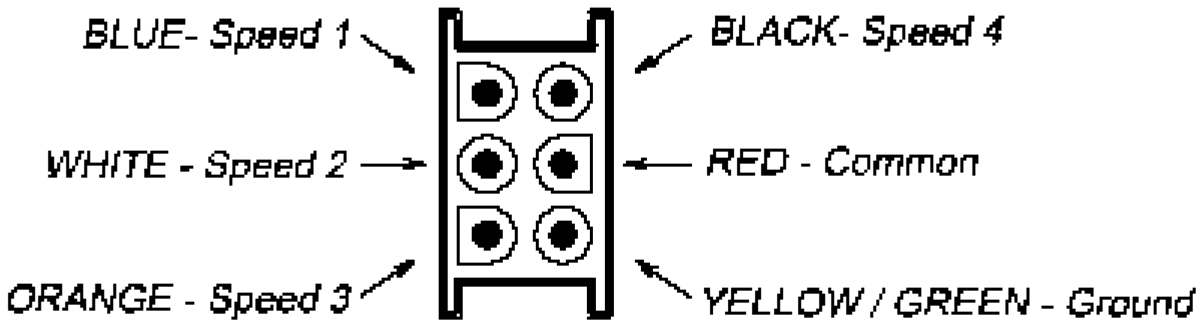
MOTOR CONNECTOR DIAGRAM
