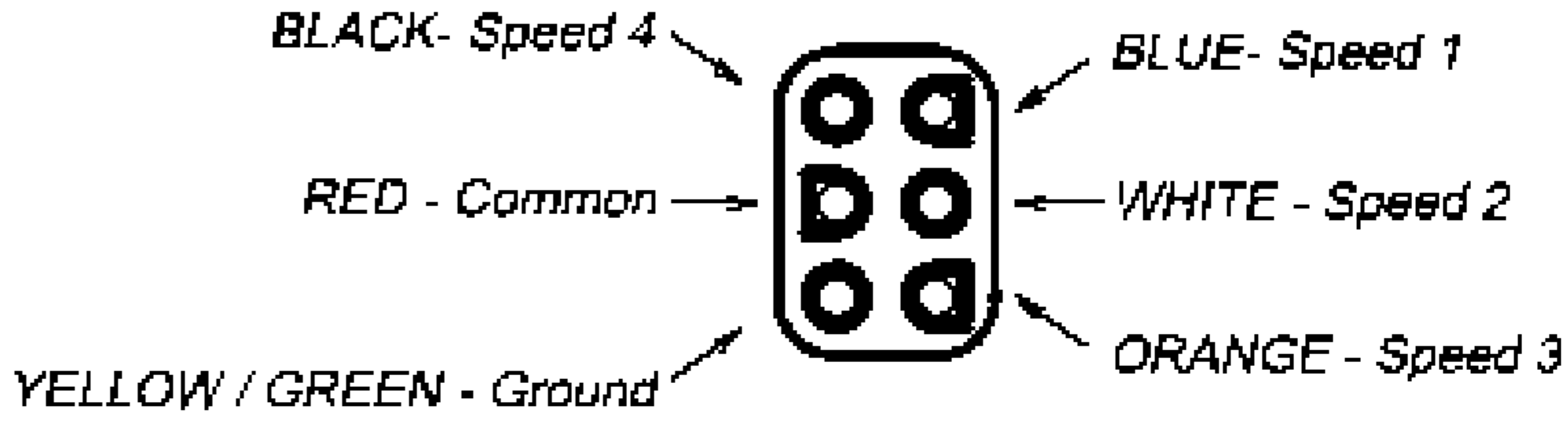
CONTROL CONNECTOR DIAGRAM
