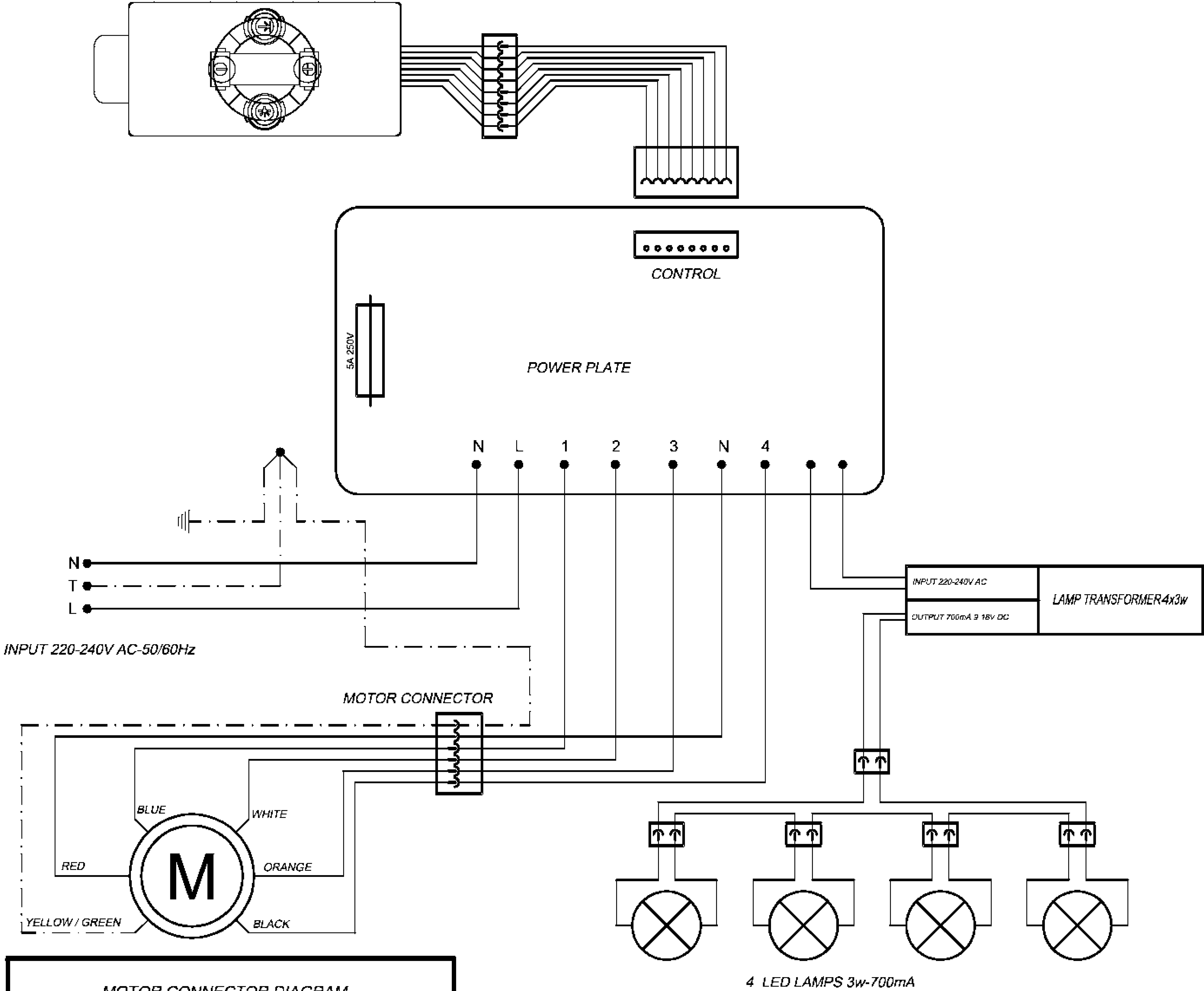
MOTOR CONNECTOR DIAGRAM
